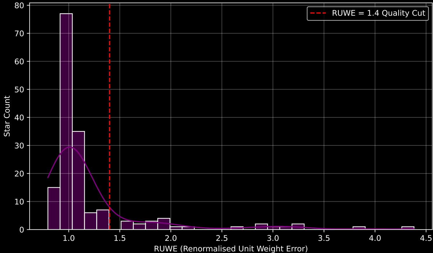
GAPOGEE DR17 Field [130+60] RUWE Distribution (n= 163)
