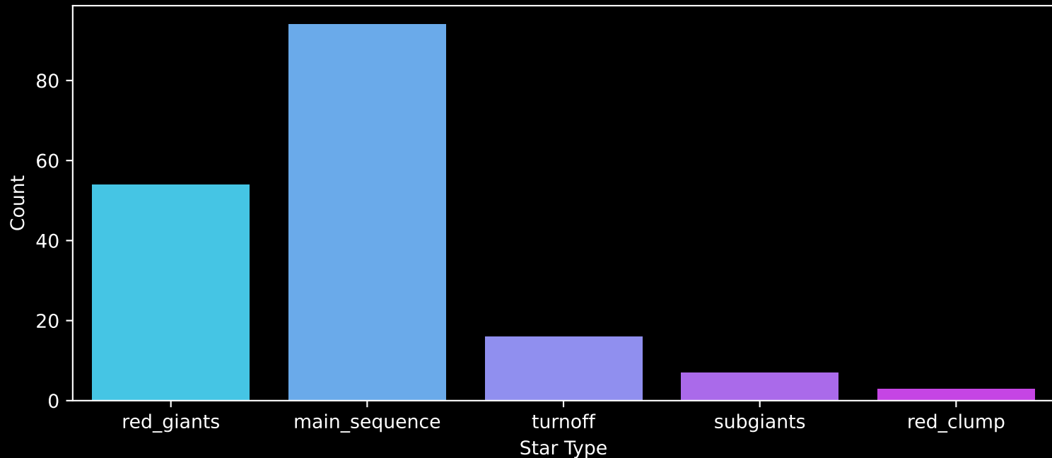
APOGEE DR17 Field: [130+60] Count plot of Star Type
