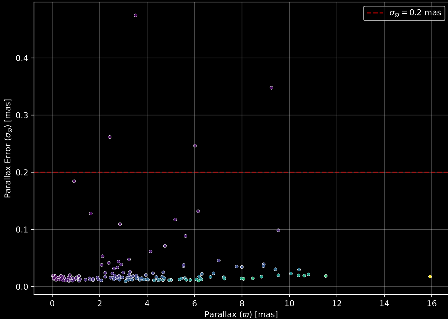
APOGEE DR17 Field: [130+60] Parallax Quality (n= 174)
