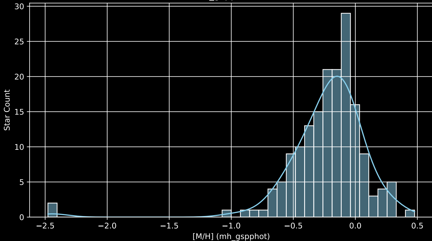
APOGEE DR17 Field: [130+60 [M/H] (mh_gspphot) (n= 171)
