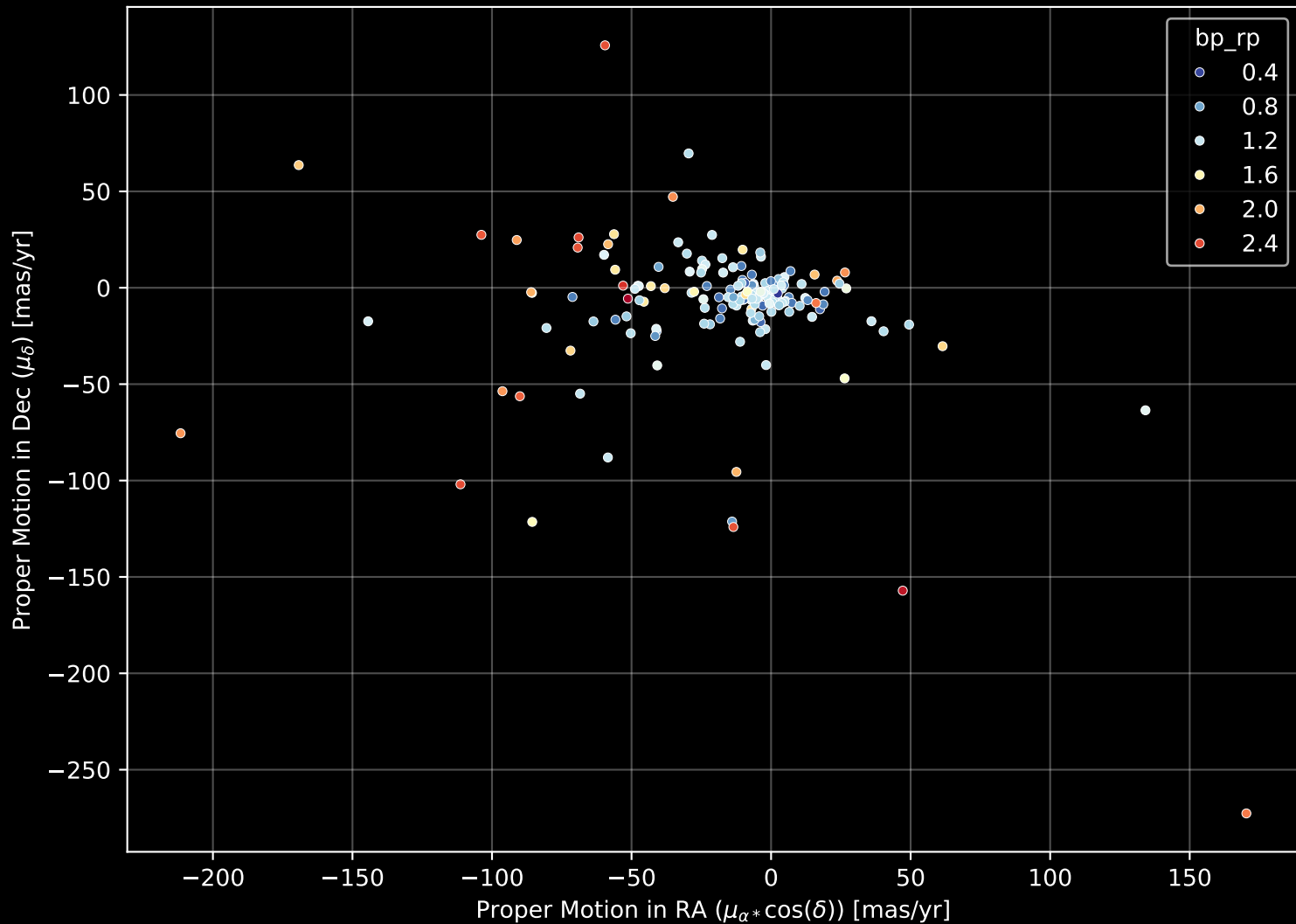
APOGEE DR17 Field: [130+60] Proper Motion Diagram (n= 174)
